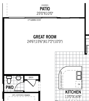
3 15' STACKED SLIDER
