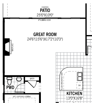
1 FIREPLACE
