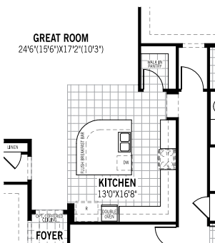
6 GOURMET KITCHEN
